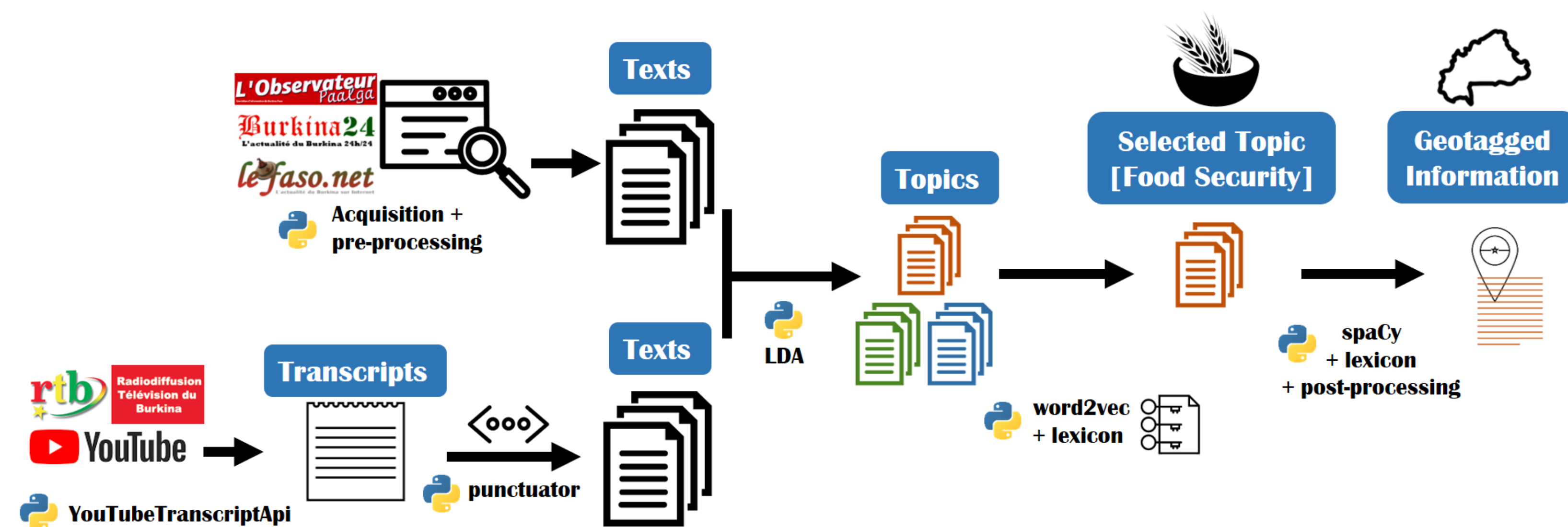
General schema of the proposed news mining framework
